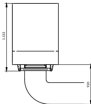
UPPER VIEW VISTA SUPERIOR
