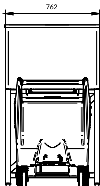
FRONTAL VIEW VISTA FRONTAL
