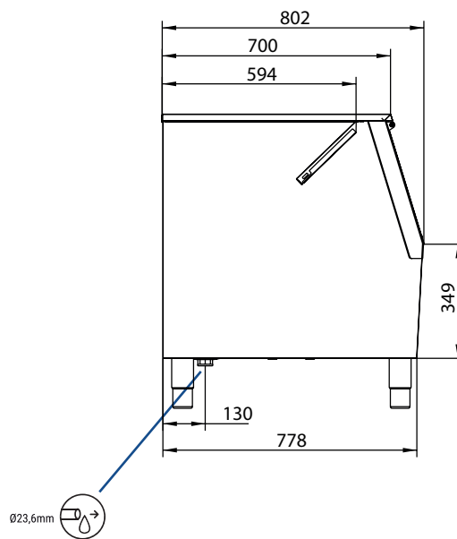
FRONTAL VIEW VISTA FRONTALE
