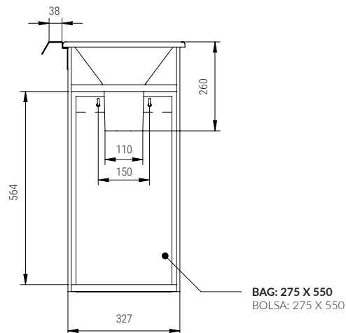
FRONTAL VIEW VISTA FRONTAL
